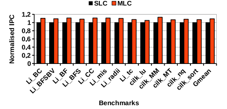
Fig. 9: Change in IPC for iso-area SLC-MRAM and MLC-MRAM LLC.
