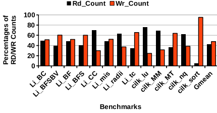
Fig. 7: Distribution of Read and Write operations.
