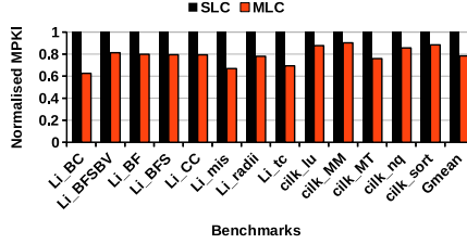
Fig. 8: Change in MPKI for iso-area SLC-MRAM and MLC-MRAM LLC.
