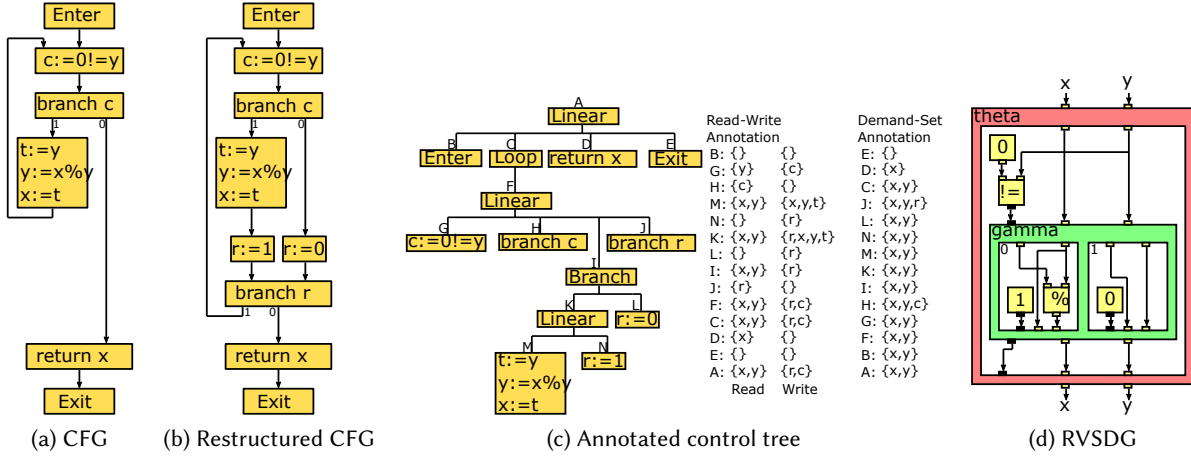
Fig. 5. Intra-Procedural Translation
