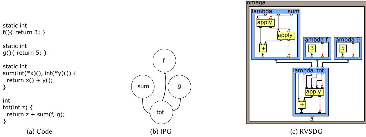
Fig. 4. Inter-Procedural Translation
